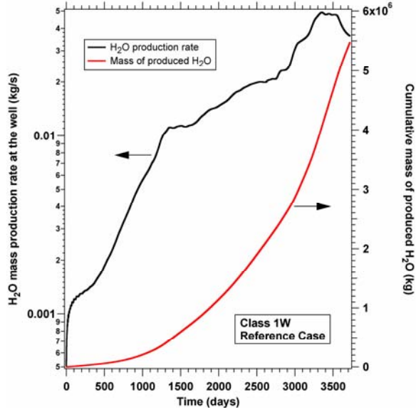
Figure 5. Water production during gas production from the Class 1W deposit in Figs. 3 and 4.
