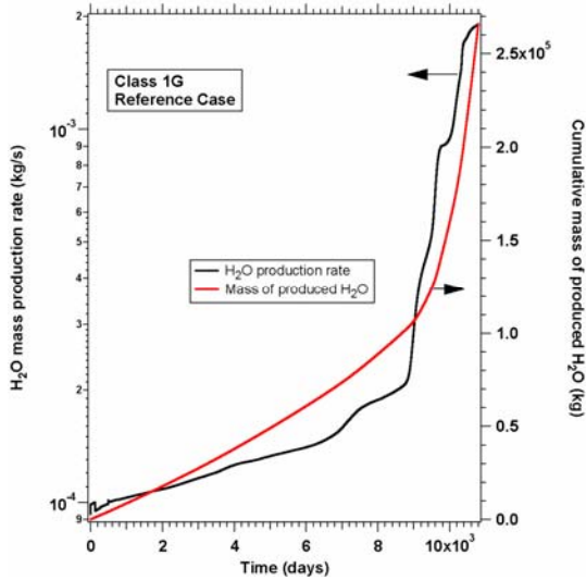
Figure 9. Water production during gas production from the Class 1G deposit in Figs. 7 and 8.
