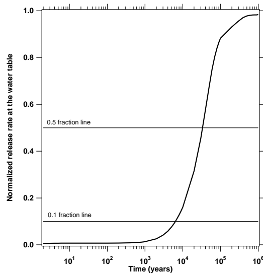
Figure 11. Normalized release rate of the ^{239}\text{Pu} chain at the UZ water table (continuous release, mean present-day infiltration).
