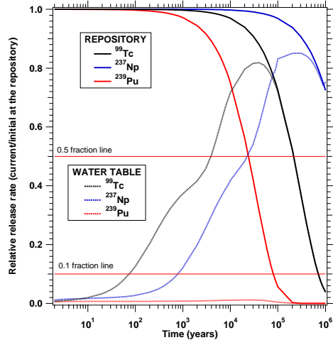
Figure 8. Normalized release rate of ^{99}\text{Tc} , ^{237}\text{Np} and ^{239}\text{Pu} at the YM water table for continuous release and mean present-day infiltration.
