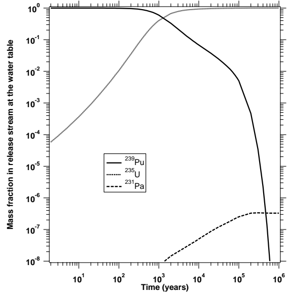
Figure 10. Mass fraction of each member of the ^{239}\text{Pu} chain in the release stream at the UZ water table.
