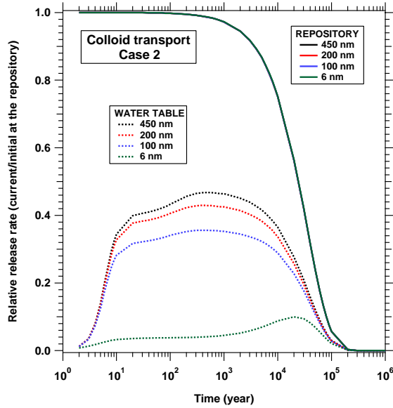
Figure 13. Case 2: Normalized release rate of colloids at the UZ water table (continuous release, mean present-day infiltration).
