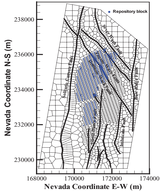
Figure 1. Plan view of the UZ model grid design at the proposed repository level
