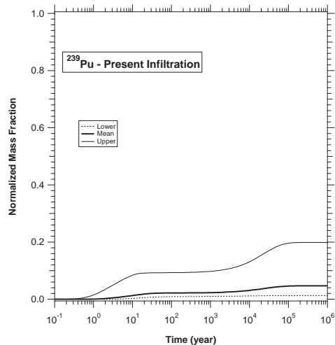
Figure 4. ^{239}\text{Pu} breakthrough at the YM water table after an instantaneous release.
