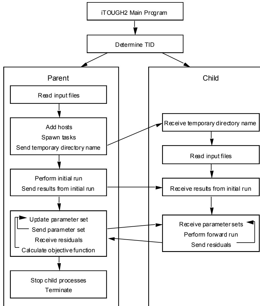
Figure B.1. Simplified iTOUGH2-PVM flow chart.
