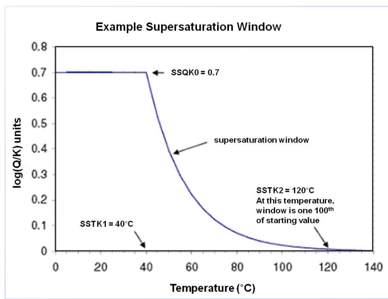
Figure B.4—2 Supersaturation window dependence on temperature.
